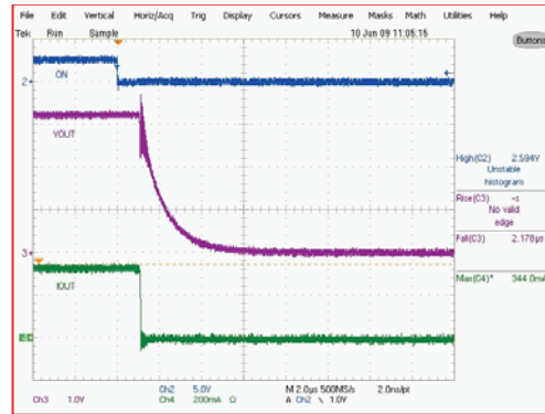
Figure 25. Turn-Off Response (V_{IN}=3.3V, C_{IN}=1\mu F, C_{OUT}=0.1\mu F, R_L=10\Omega)
