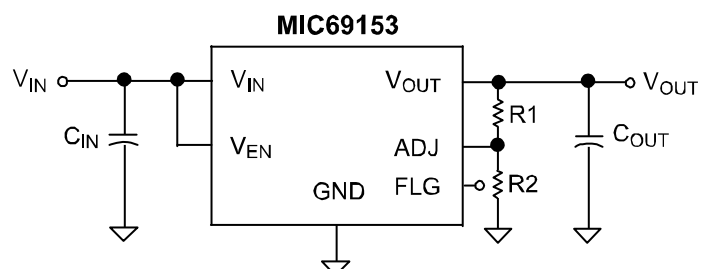
Adjustable Regulator
