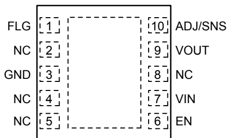
10-Pin 3mm x 3mm MLF ® (ML)
