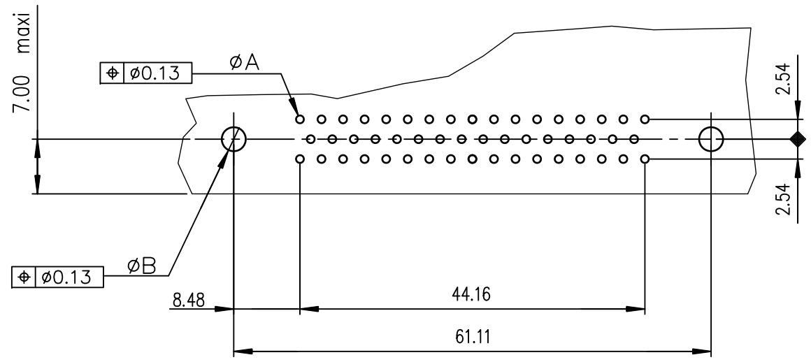
PC card drilling dimensions(after plating) scale:1.5 (thickness 1.60 ±0.10mm)
