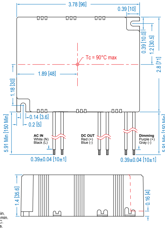
“-SY” Optional Side Leads Configuration:
