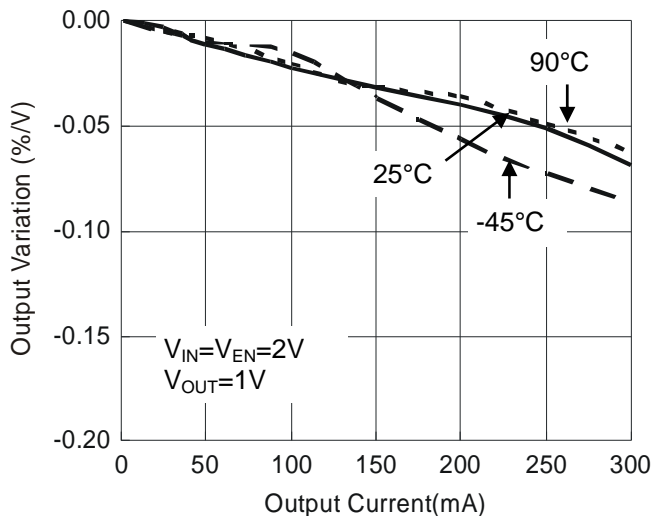
Load Regulation
