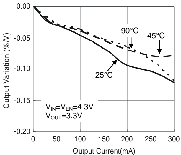
Load Regulation
