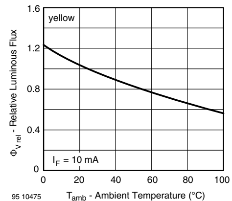
Fig. 18 - Relative Luminous Flux vs. Ambient Temperature
