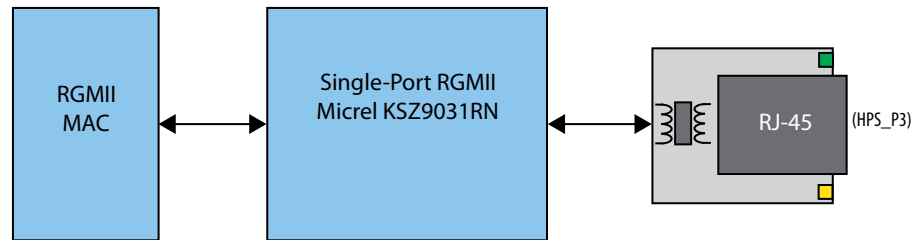
Figure 5-5: RGMII Interface between HPS (MAC) and PHY
