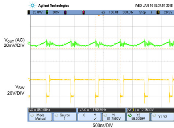
Figure 7. Output Voltage Ripple ( V_{IN} = 28V , V_{OUT} = 24V , 4A Load)
