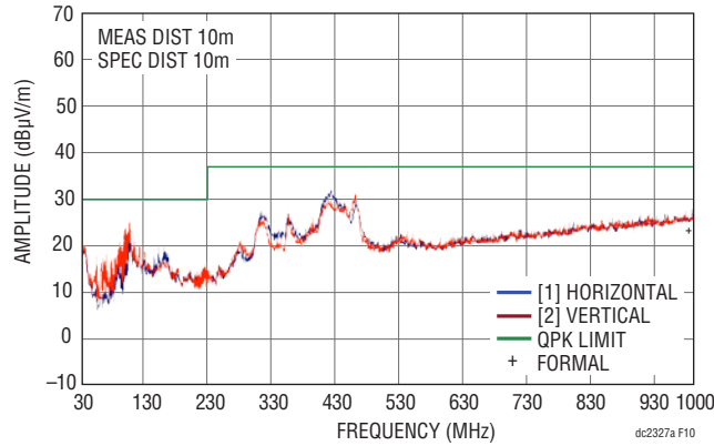
Figure 10. Radiated Emissions Scan of the LTM4653. Producing 24V OUT at 4A, from 29.5V IN . DC2327A Hardware. f SW = 1.2MHz. Measured in a 10m Chamber. Peak Detect Method
