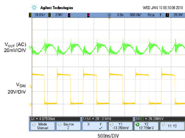
Figure 8. Output Voltage Ripple ( V_{IN} = 48V , V_{OUT} = 24V , 4A Load)
