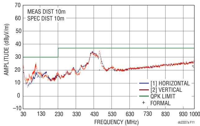
Figure 11. Radiated Emissions Scan of the LTM4653 Producing 24V OUT at 3.5A, from 48V IN . DC2327A Hardware. f SW = 1.2MHz. Measured in a 10m Chamber. Peak Detect Method
