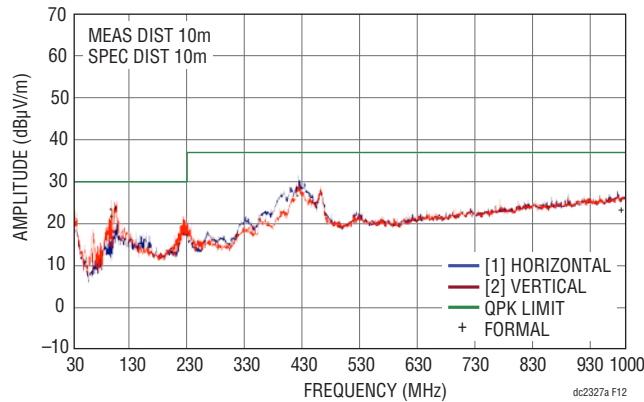
Figure 12. Radiated Emissions Scan of the LTM4653. Producing 12V OUT at 3A, from 58V IN . DC2327A Hardware. f SW = 1.2MHz. Measured in a 10m Chamber. Peak Detect Method
