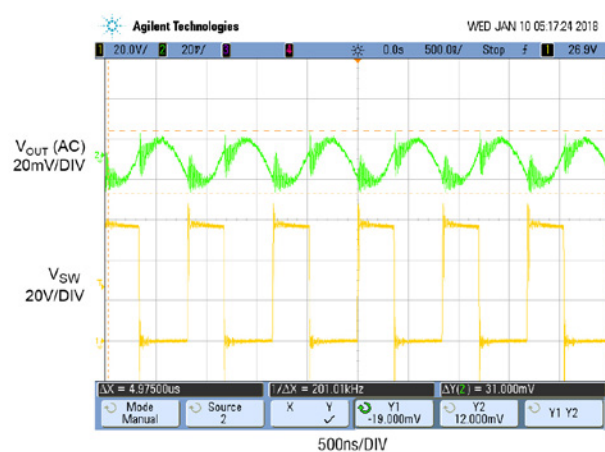
Figure 9. Output Voltage Ripple ( V_{IN} = 58V , V_{OUT} = 24V , 4A Load)
