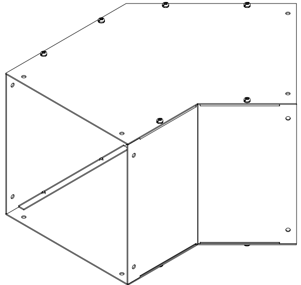
ISOMETRIC VIEW
