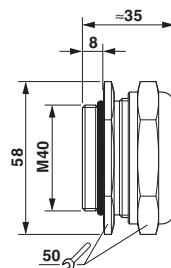
Dimensional drawing
