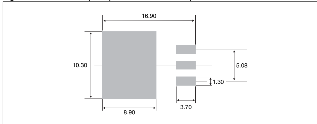
Figure 14. D 2 PAK footprint (all dimensions in mm)
