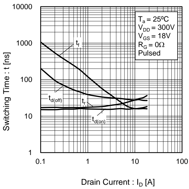
Fig.17 Switching Characteristics
