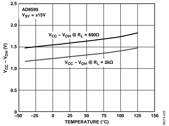
Figure 27. Output Saturation Voltage vs. Temperature
