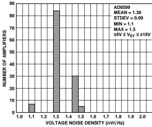
Figure 40. Voltage Noise Density at 10 Hz
