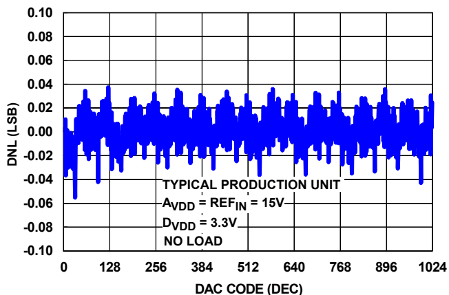
FIGURE 16. DAC1-DAC15 DNL ( \text{REF}_{\text{IN}} = \text{A}_{\text{VDD}} = 15\text{V} ) AT +25^\circ\text{C}
