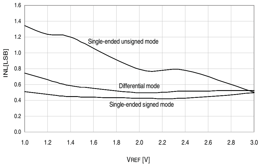
Figure 34-312. INL Error vs. External V_{REF} T = 25\text{ }^{\circ}\text{C} , V_{CC} = 3.6\text{V} , external reference
