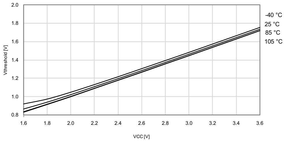
Figure 34-170. I/O Pin Input Threshold Voltage vs. V_{CC}
