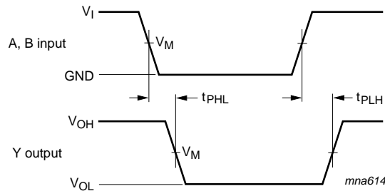
Measurement points are given in Table 10 . Logic levels: V OL and V OH are typical output voltage drops that occur with the output load.
