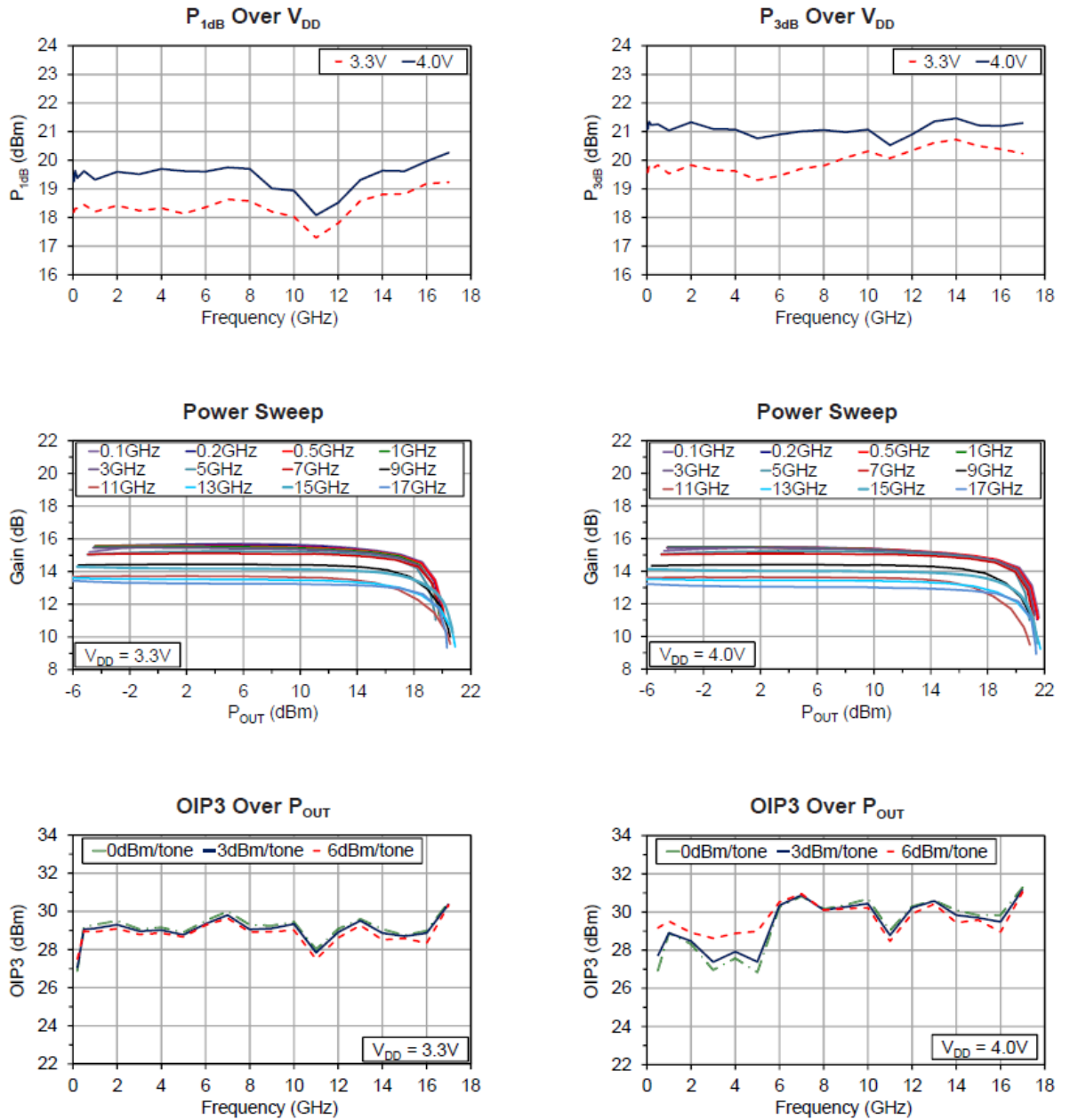
Figure 4 P 1dB /P 3dB , OIP3, and Power Sweep
