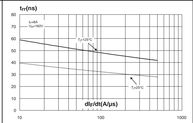
Figure 8. Reverse recovery time versus dl_F/dt (typical values, per diode)
