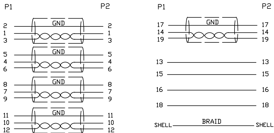
1.Wiring Diagram.
