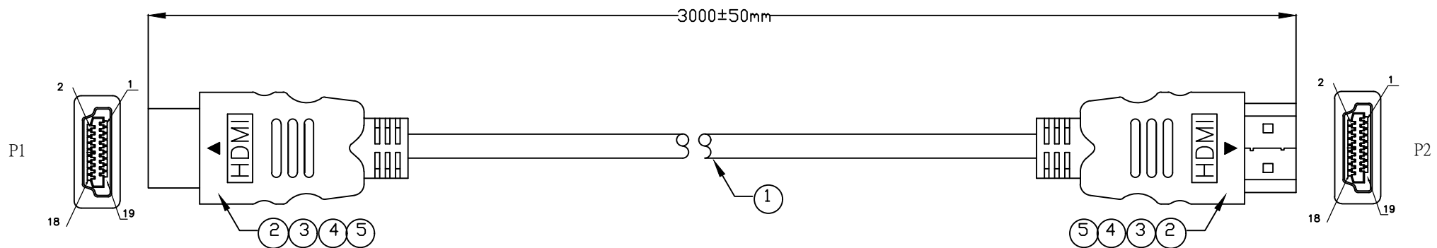
1.Wiring Diagram.
