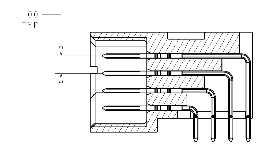
SECTION Z-Z
