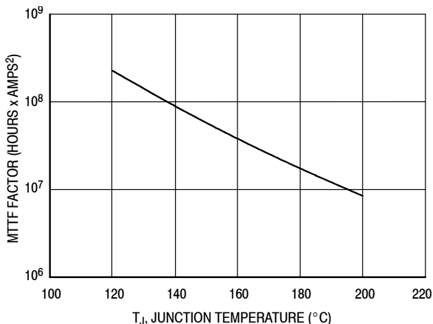
This above graph displays calculated MTTF in hours x ampere 2 drain current. Life tests at elevated temperatures have correlated to better than \pm 10\% of the theoretical prediction for metal failure. Divide MTTF factor by I_D^2 for MTTF in a particular application.
