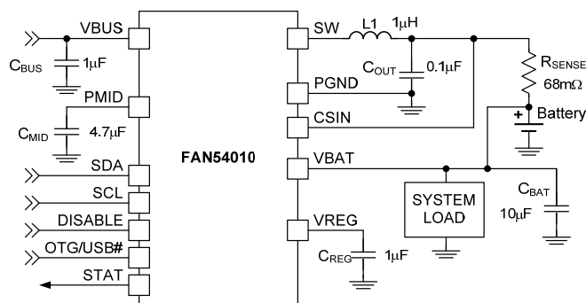
Figure 1. Typical Application
