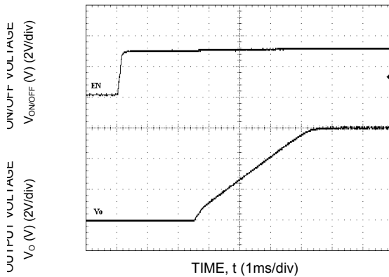
Figure 41. Typical Start-up Using On/Off Voltage (I o = I o,max ).
