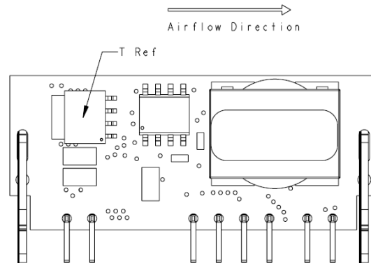
Figure 53. Temperature measurement location T_{ref} .
