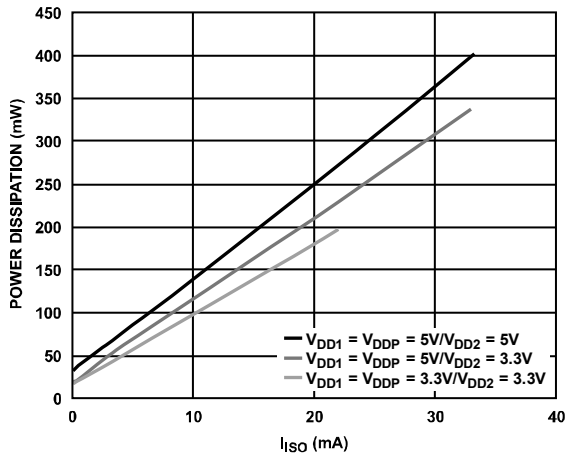
Figure 7. Total Power Dissipation vs. Output Supply Current, I_{SO} , with Data Channels Idle
