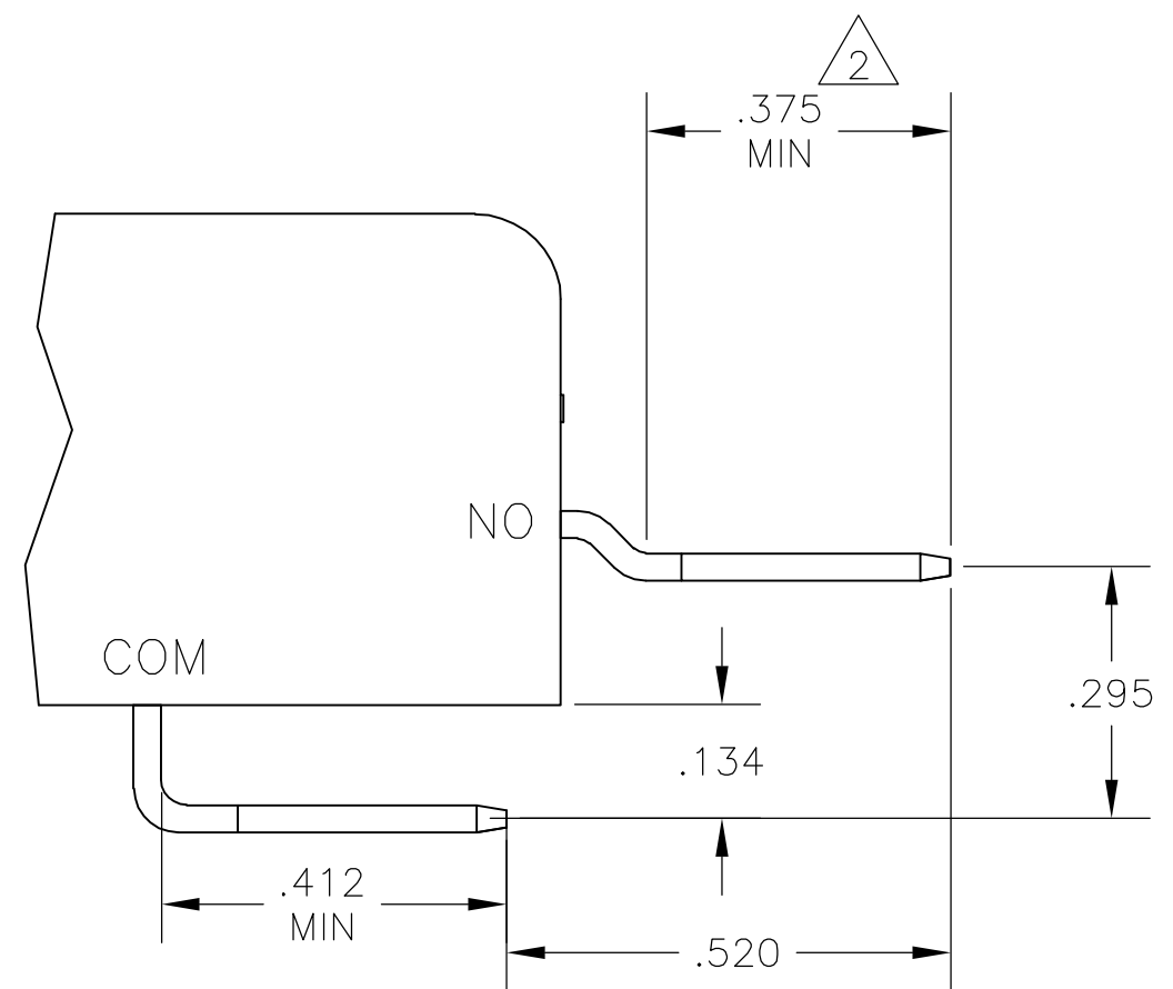
MATING SWITCH VIEW
