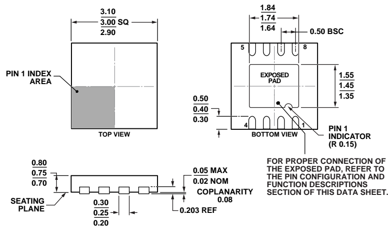
Figure 78. 8-Lead Lead Frame Chip Scale Package [LFCSPP] 3 mm x 3 mm Body and 0.75 mm Package Height (CP-8-13)
