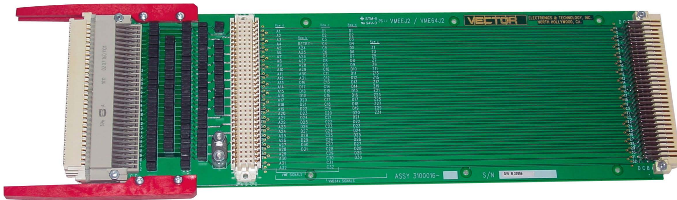
3U, VME64x J2 with 5-row, 160 positions DIN 41612 style connectors (click on image to enlarge)
