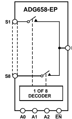
SWITCHES SHOWN FOR A LOGIC 1 INPUT.
