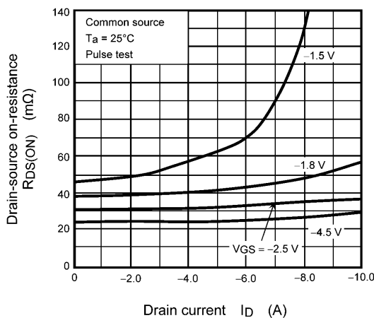
Fig. 7.5 R_{DS(ON)} - I_D
