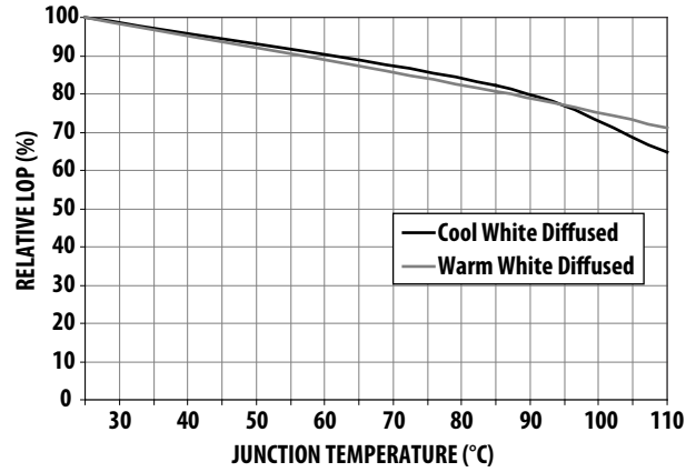
Figure 7. Relative LOP vs. junction temperature
