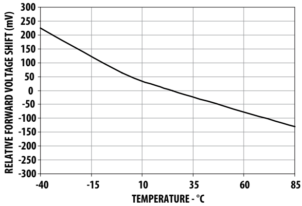
Figure 6. Temperature vs. relative forward voltage shift
