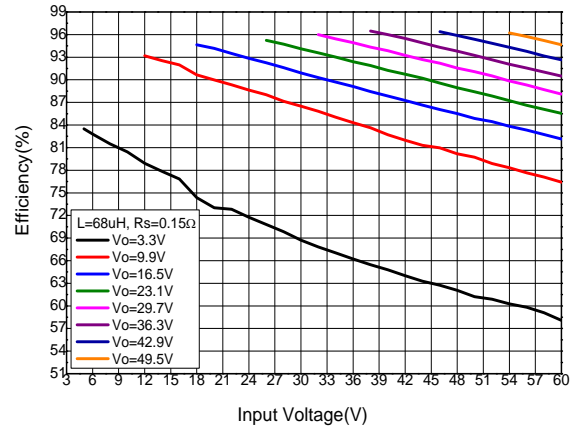
Efficiency vs. Input Voltage ( R_s=0.15\Omega , L=68\mu\text{H} )
