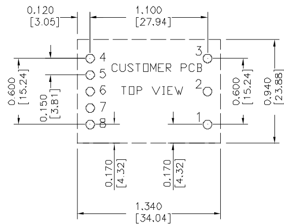
RECOMMENDED PCB PAD LAYOUT
