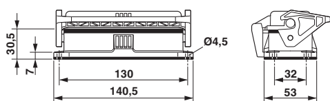
Dimensional drawing
