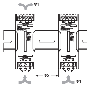
(A) Standard (Vertical) mounting
