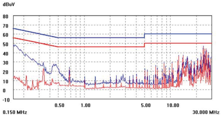
Figure 25. EMC Considerations
