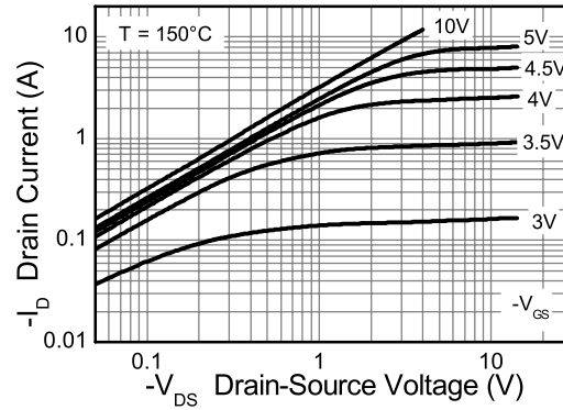
Output Characteristics
