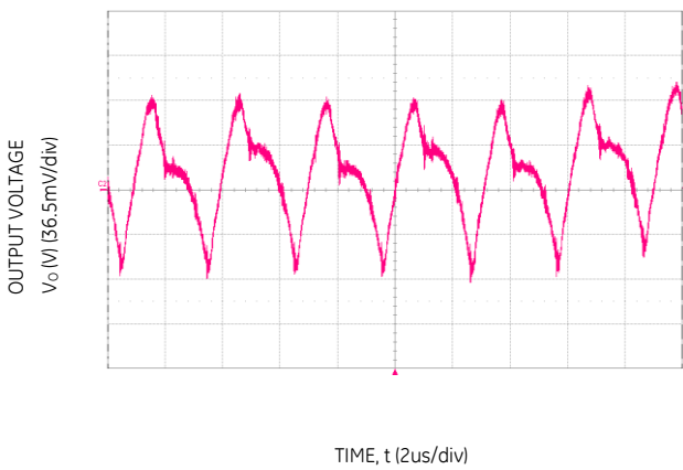
Figure 3. Typical output ripple and noise (C o =3x10uF+470uF, V IN = 12V, I o = I o,max ).
