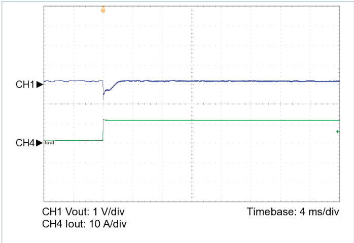
Figure 6 — 10% to 100% load transient response, V_{IN} = 48\text{ V} , nominal trim, C_{OUT\_EXT} = 250\ \mu\text{F}
