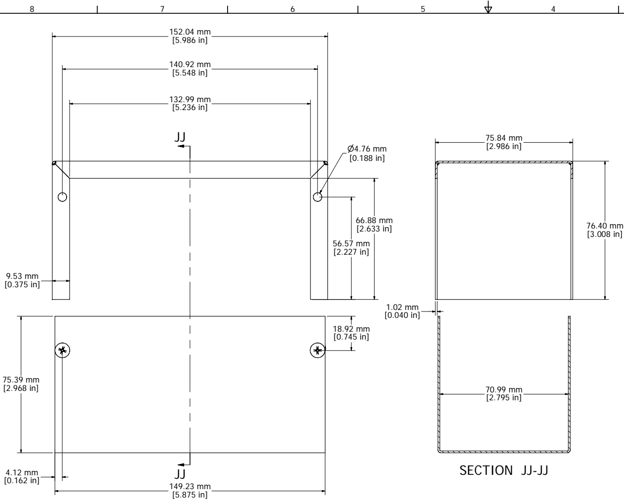
ASSEMBLY - VIEW FROM SIDE (OPEN)
