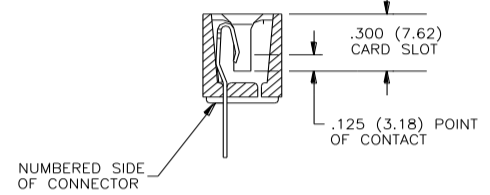
SINGLE ROW CONTACTS READ ONE SIDE OF DAUGHTER BOARD
