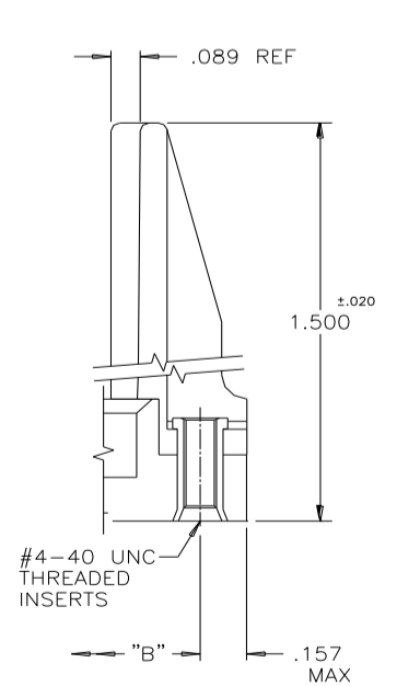
MOUNTING OPTION CODE #78
