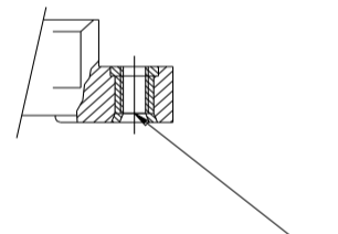
VARIATIONS 07 AND 08 THREADED INSERT
