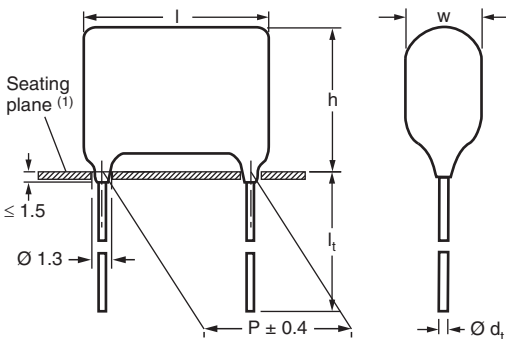
469 Straight Leads
