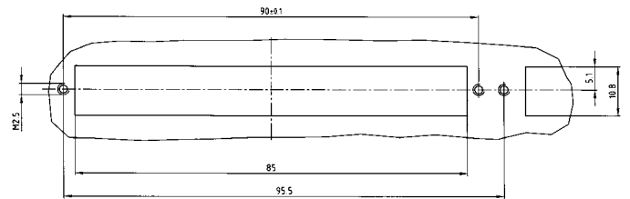
Panel cutout
