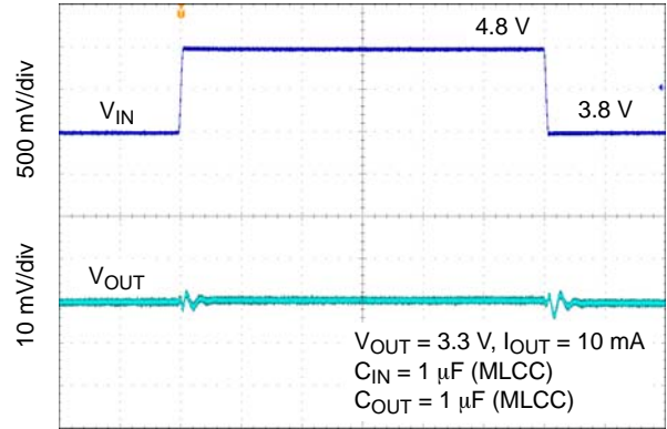
Figure 38. Line Transient Response – V_{OUT} = 3.3 \text{ V}
