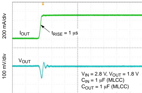
Figure 41. Load Transient Response – 1 mA to 450 mA – V_{OUT} = 1.8 \text{ V}
