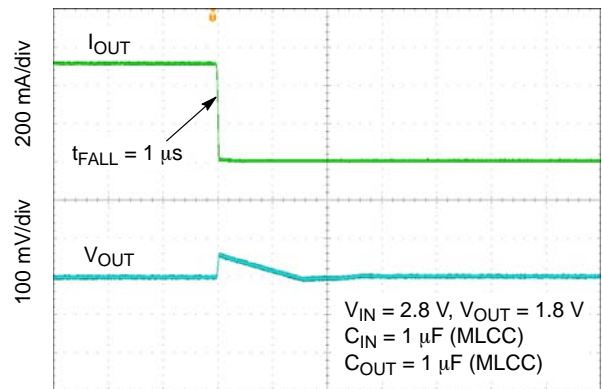
Figure 42. Load Transient Response – 450 mA to 1 mA – V_{OUT} = 1.8 \text{ V}
