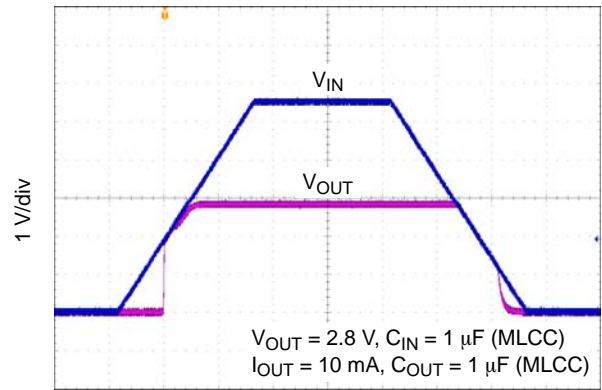
Figure 40. Turn-on/off – Slow Rising V_{IN}
