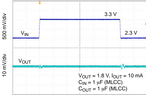
Figure 37. Line Transient Response – V_{OUT} = 1.8 \text{ V}
