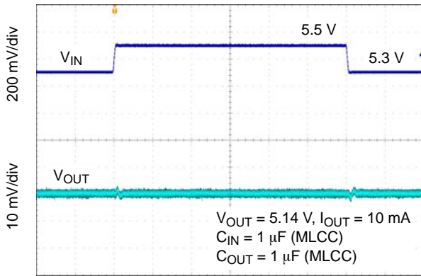
Figure 39. Line Transient Response – V_{OUT} = 5.14 \text{ V}
