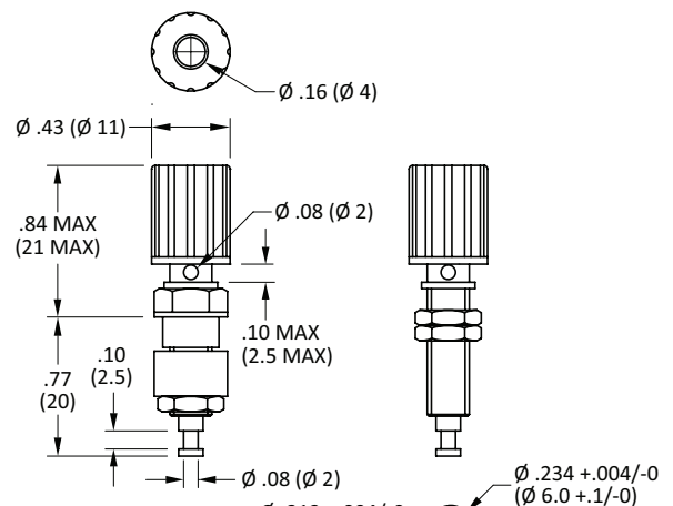
MOUNTING HOLE
