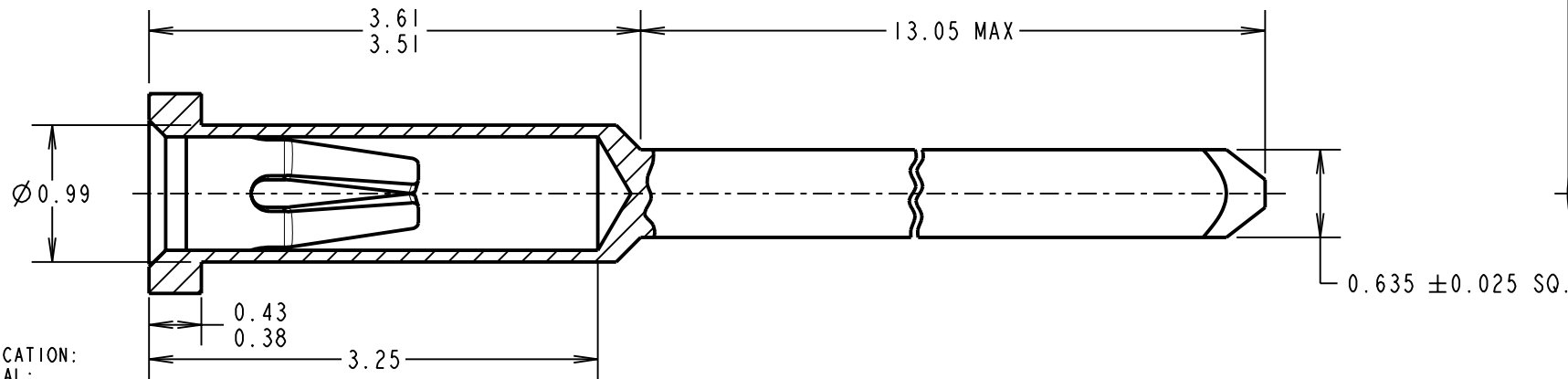
PART SECTION X-X
