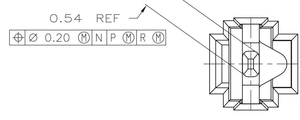
VIEW W-W SCALE 20:1
