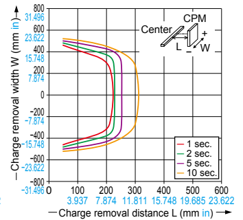
Charge removal field (vertical direction, airless, 10 Hz)
