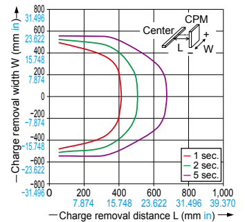
Charge removal field (vertical direction, 0.005 MPa, 1 Hz)
