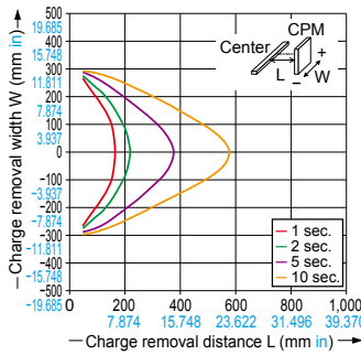
Charge removal field (vertical direction, 0.005 MPa, 50 Hz)
