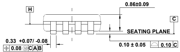
SIDE VIEW 1
