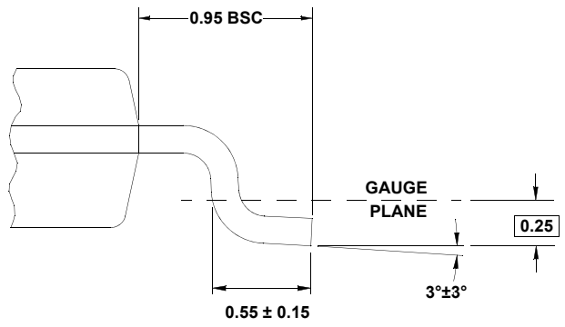
DETAIL "X"
