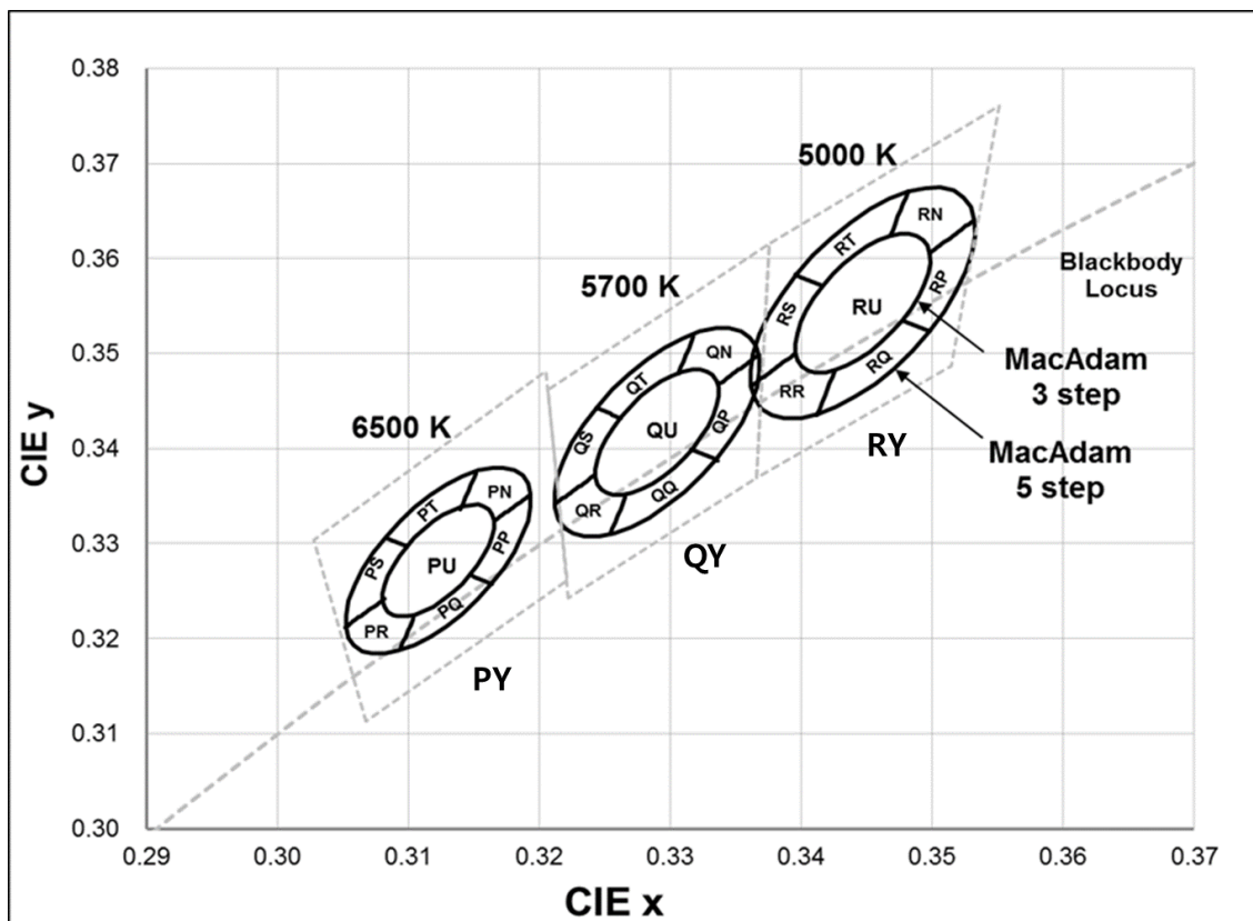
f) Chromaticity Region & Coordinates ( I_f = 150 \text{ mA} , T_s = 25 \text{ }^\circ\text{C} )
