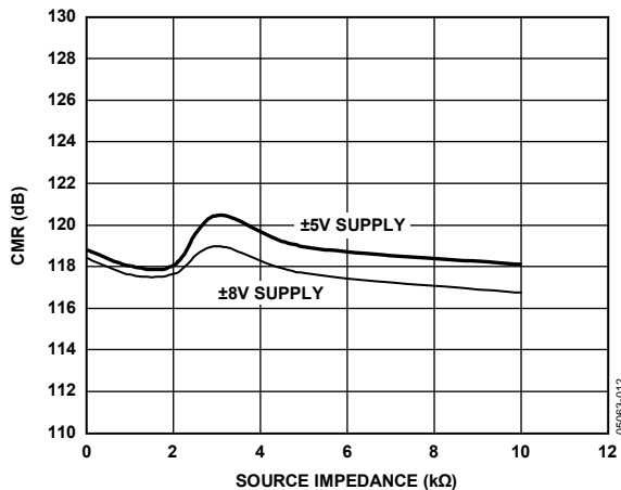
Figure 12. Common-Mode Rejection (CMR) vs. Source Impedance, 1.1 µF Across Input Pins
